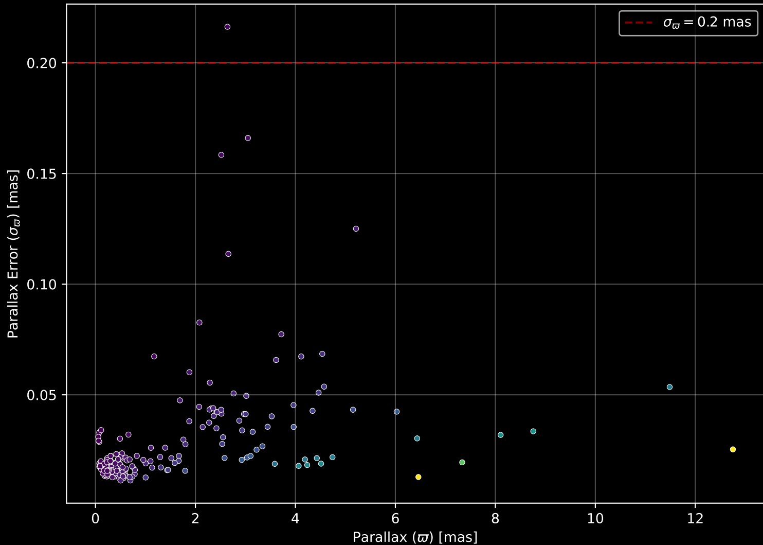
APOGEE DR17 Field: [169+24_btx] Parallax Quality (n= 190)
