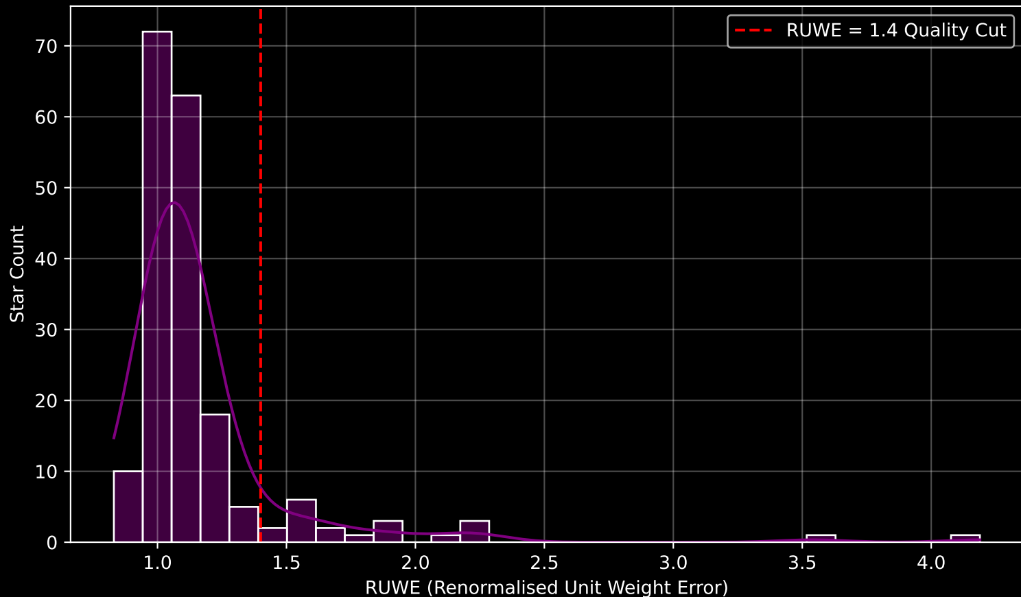
GAPOGEE DR17 Field [169+24_btx] RUWE Distribution (n= 188)
