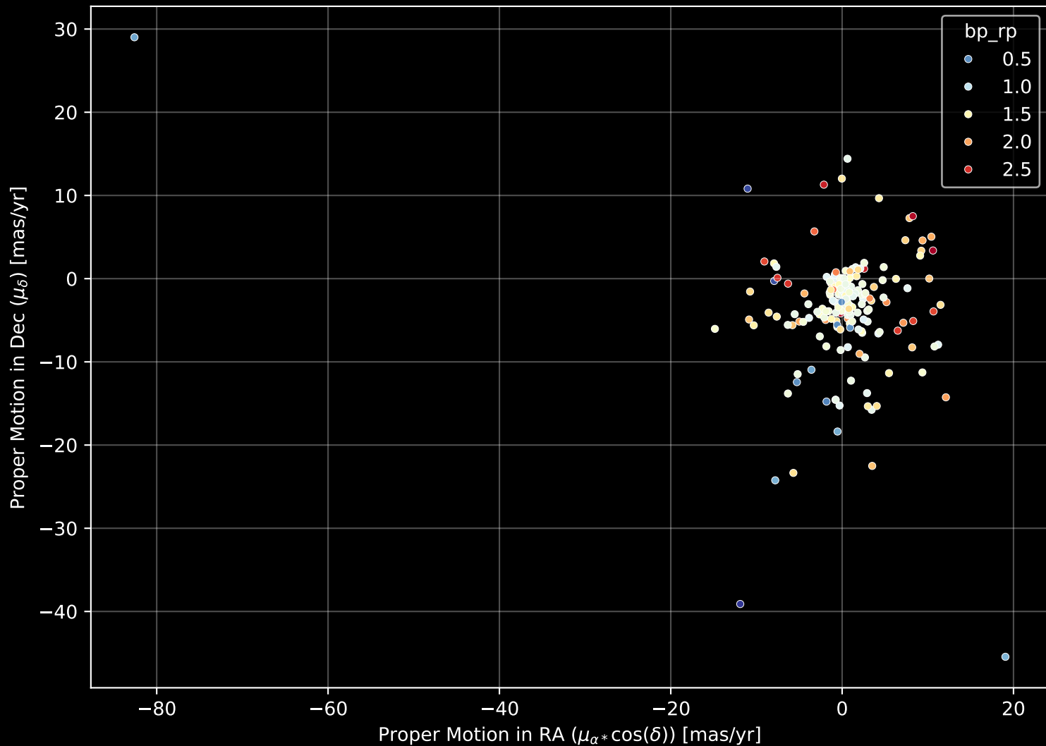
APOGEE DR17 Field: [169+24_btx] Proper Motion Diagram (n= 190)
