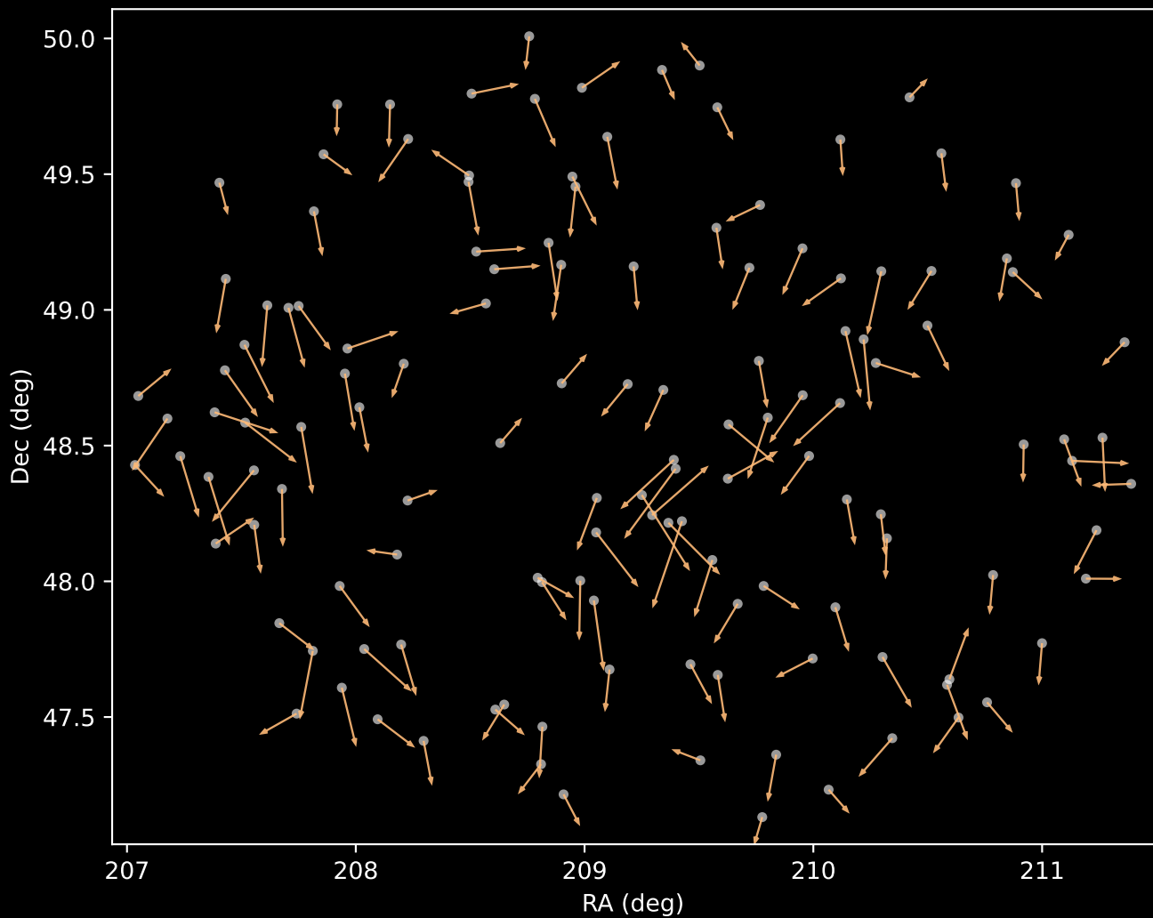
APOGEE DR17 Cluster 3 Proper Motion Vectors (n=134)
