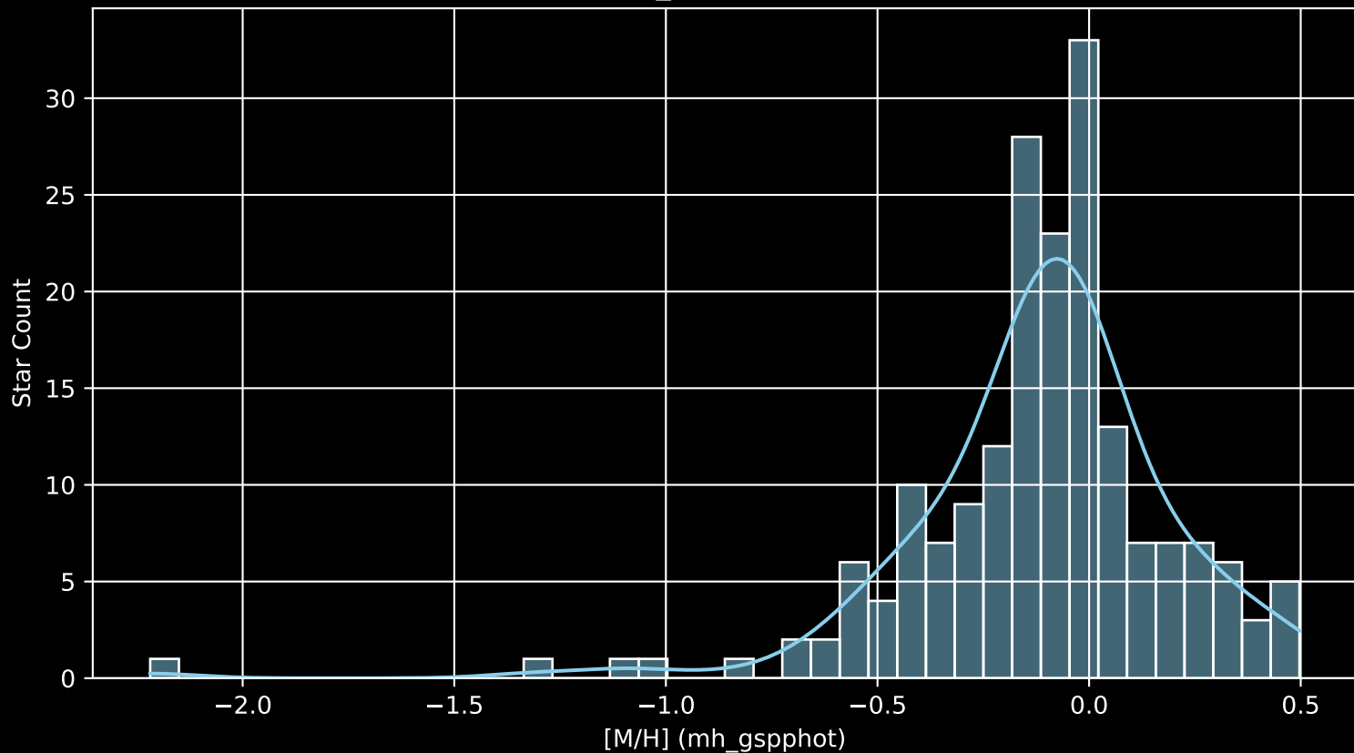
APOGEE DR17 Field: [169+24_btx [M/H] (mh_gspphot) (n= 189)
