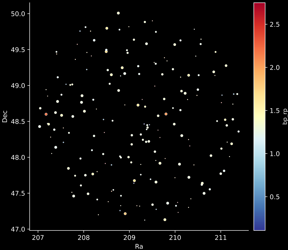
APOGEE DR17 Field: [169+24_btx] Stars: 190
